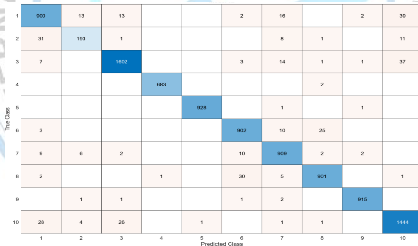
Figure 5. Confusion matrix of decision trees method for one sensor
