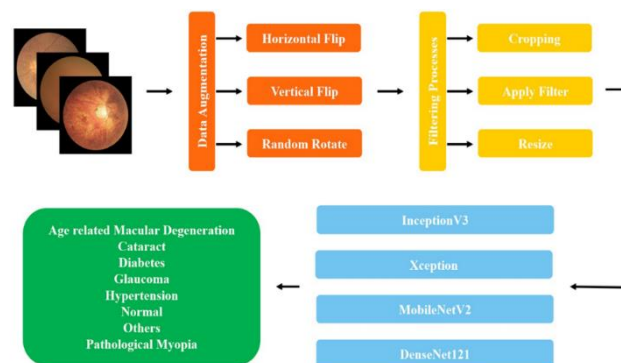
Figure 21. Workflow of the proposed system
