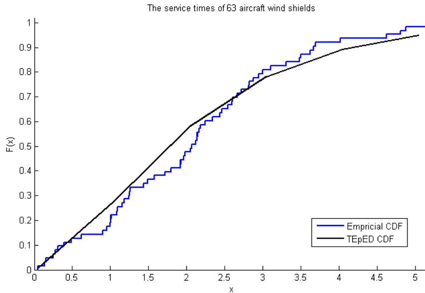
Figure 3: Empirical and TEpED distributions based on the first data set.
