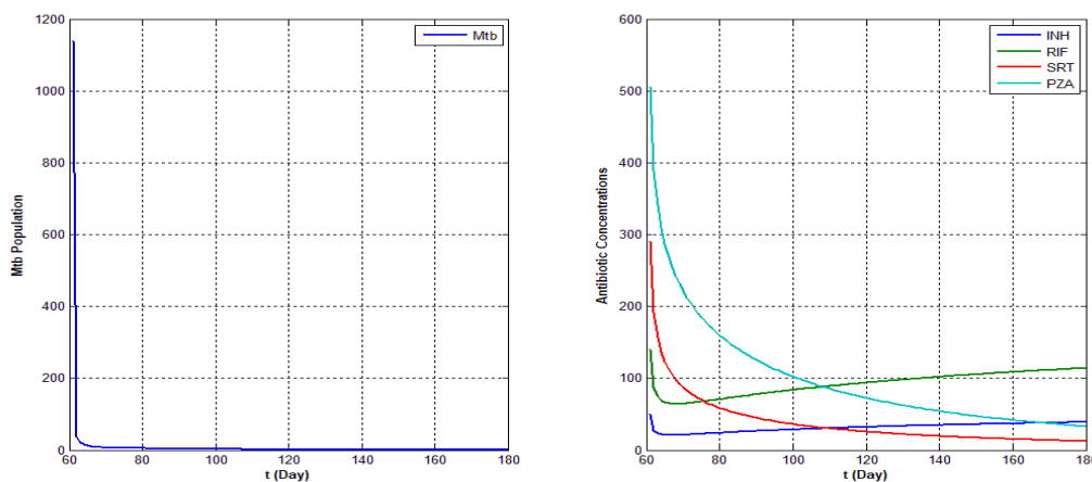
Figure 4. Time-dependent changes of variables in the proposed model in the last 4 months of treatment, including INH, RIF, SRT and PZA, for Mtb
