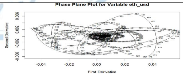
Figure 4.2.Ethereum Phase Plane
