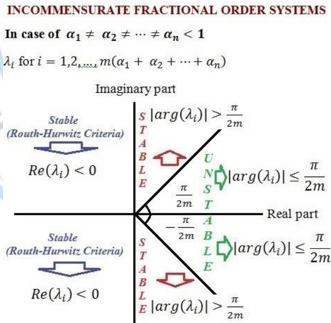
Figure 1. Analysis of eigenvalues for IFOS in Eqs. (6) (Daşbaşı, 2020).
