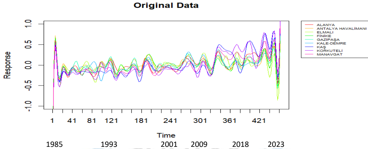
Figure 2. Monthly Maximum Temperature Curves
